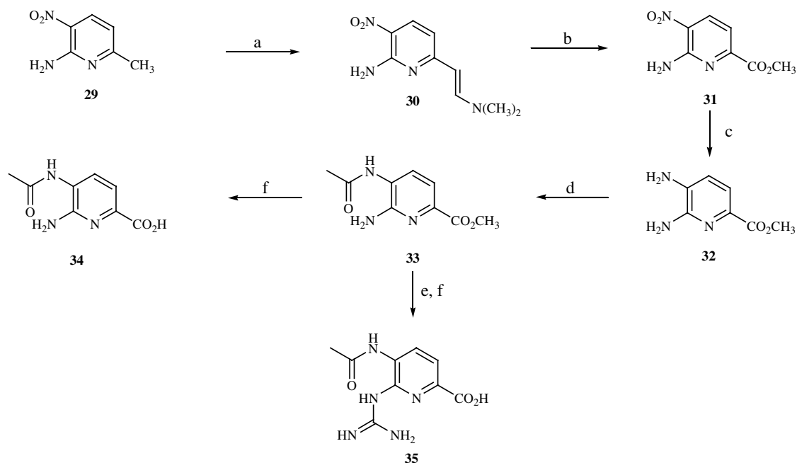
Scheme 4. Reagents and conditions: (a) (\text{CH}_3\text{O})_2\text{CHN}(\text{CH}_3)_2 , DMF; (b) (1) \text{KMnO}_4 , \text{K}_2\text{CO}_3 , aq tert -BuOH; (2) \text{MeOH} , \text{H}_2\text{SO}_4 ; (c) \text{H}_2/\text{PtO}_2 ; (d) \text{Ac}_2\text{O} , pyridine; (e) \text{H}_2\text{NCN} , \text{HCl} , \text{EtOAc} ; (f) \text{NaOH} , \text{H}^+ .
