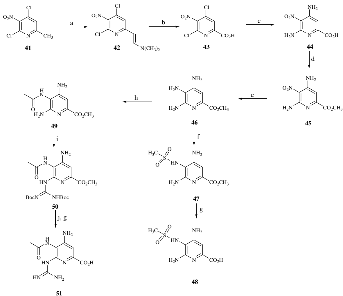
Scheme 6. Reagents and conditions: (a) (CH 3 O) 2 CHN(CH 3 ) 2 , DMF; (b) KMnO 4 , K 2 CO 3 , aq tert -BuOH; (c) NH 3 /MeOH; (d) MeOH, H 2 SO 4 ; (e) H 2 /PtO 2 ; (f) CH 3 SO 2 Cl, pyridine; (g) NaOH, H + ; (h) Ac 2 O, pyridine; (i) BocHNC(=S)NHBoc, HgCl 2 , TEA; (j) CF 3 CO 2 H, CH 2 Cl 2 .
