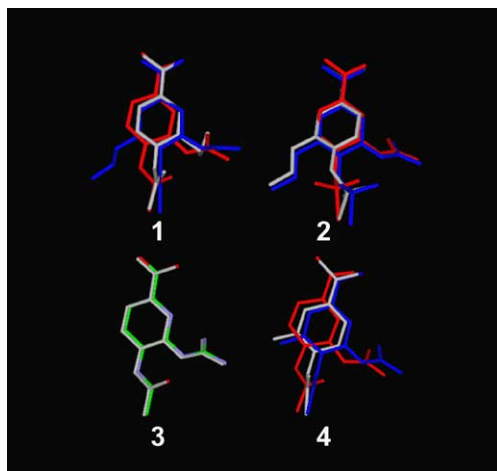
Figure 1. X-ray crystal structure of compounds in the active site of N9 neuraminidase (1) 5a (red), 5b (gray) and 12 (blue). (2) 7b (red), 5d (gray) and 21 (blue). (3) 5a (gray) and 35 (green). (4) 5a (red), 5e (gray) and 51 (blue).
